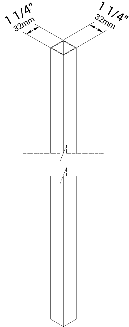
Middle Rail
