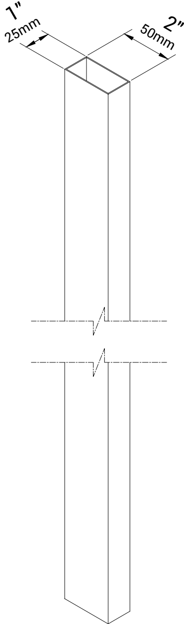
Top Rail
